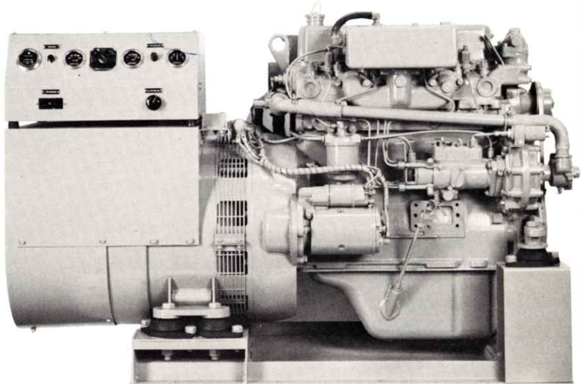
Shown here is the BR series generator, available in 30 or 45 KW capacities.
