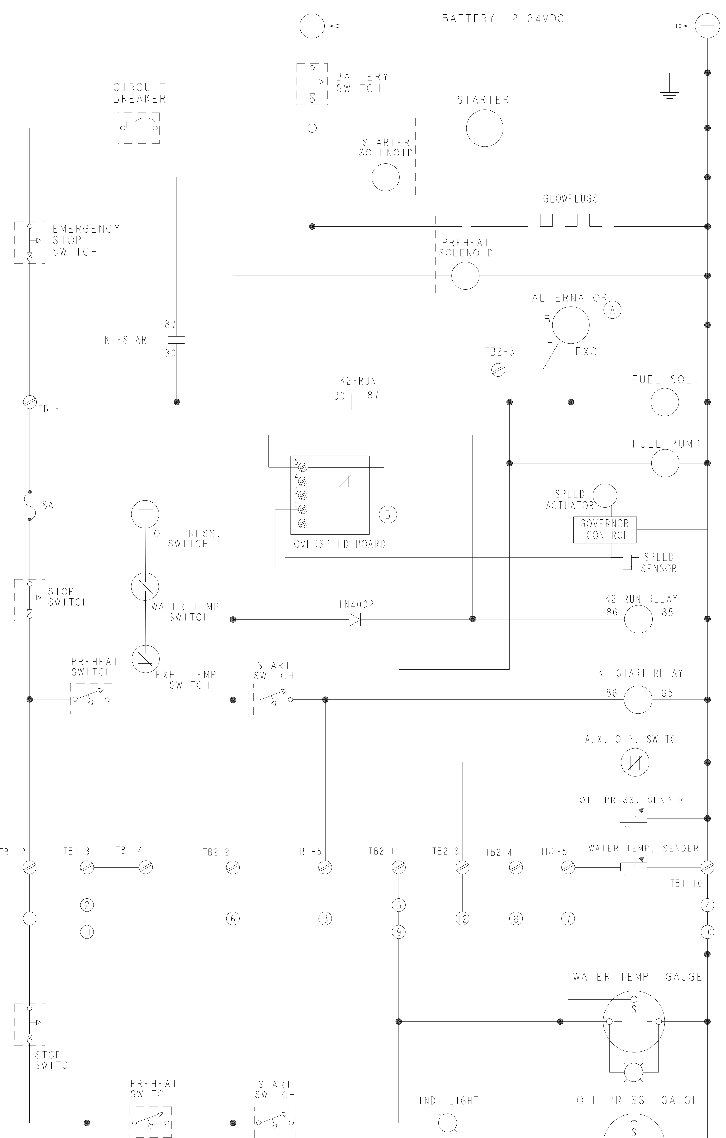
-TYPICAL REMOTE START/STOP PANEL CONNECTIONS-
